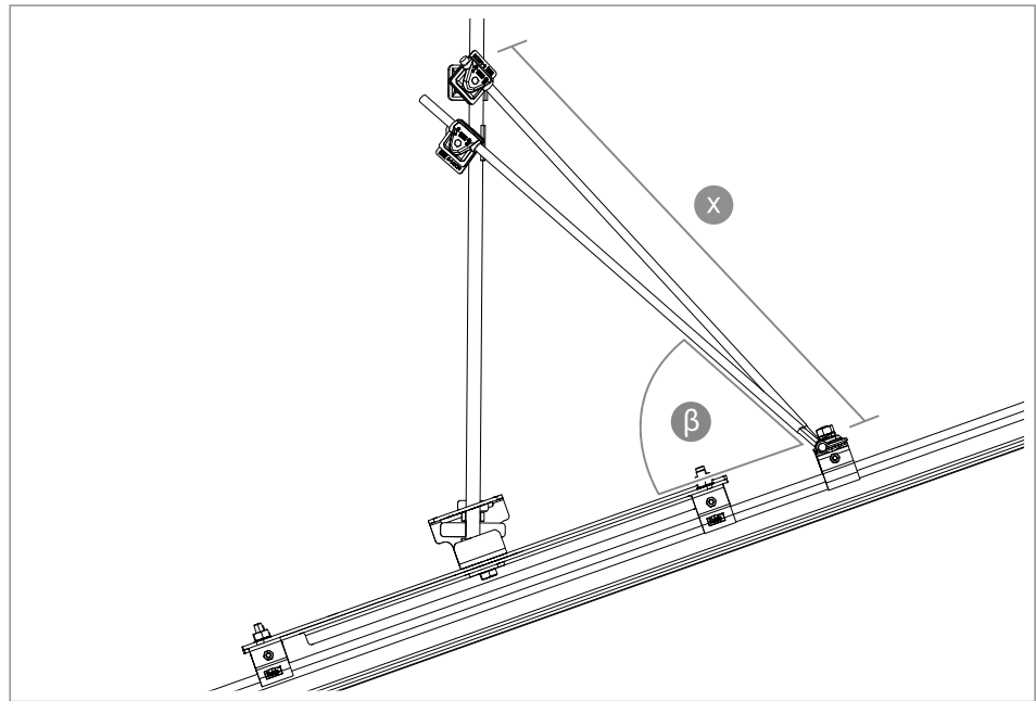
Fig. 13: Angle and length
