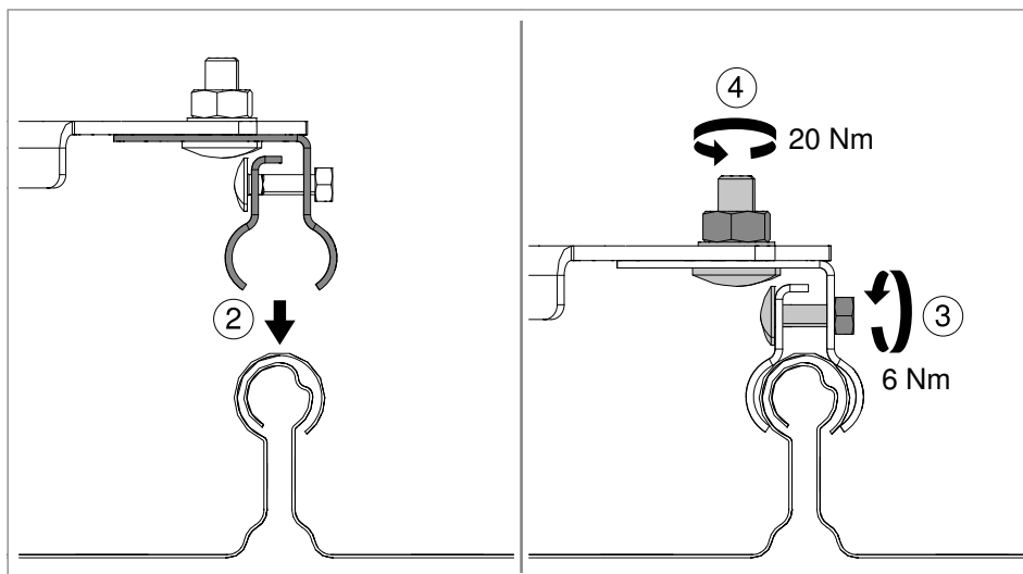
Fig. 4: Fastening the clamps
