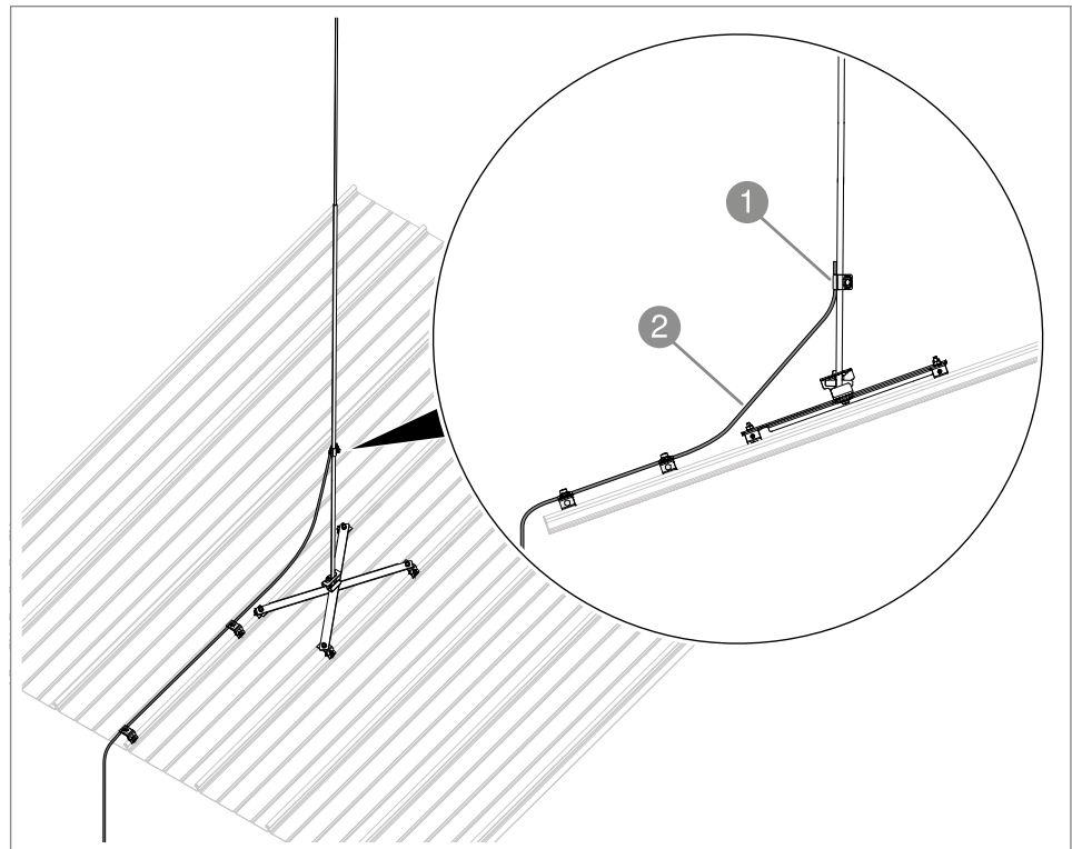
Fig. 9: Attaching the down conductor
