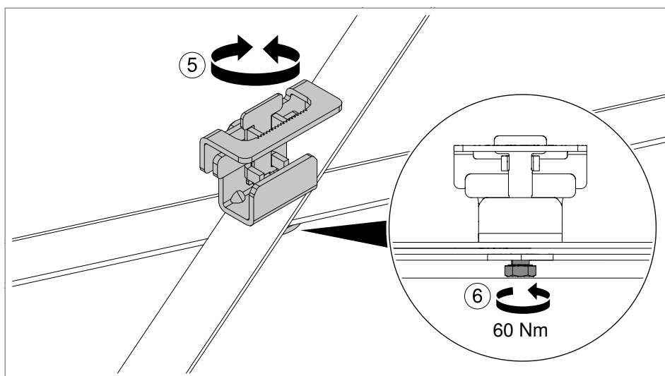
Fig. 5: Aligning the clamping element
